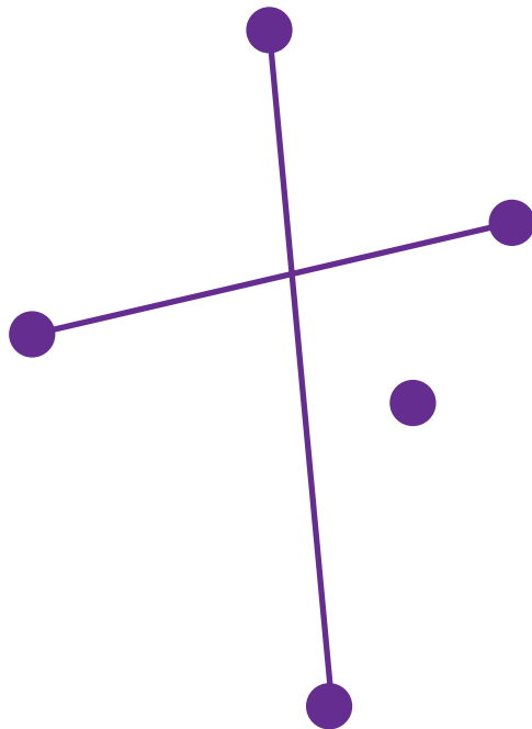
CRUX (The Southern Cross)
