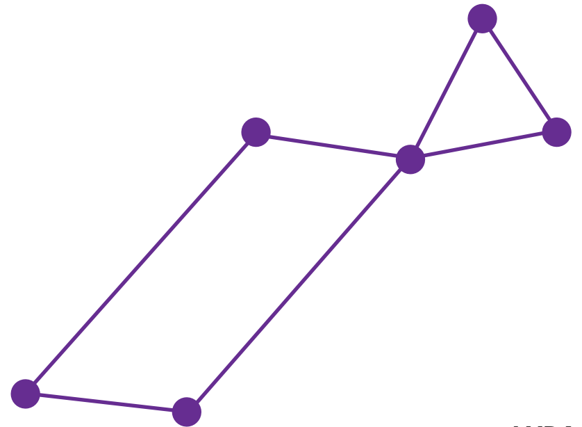
LYRA (The Lyre - a musical instrument)
