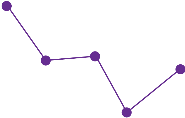
CASSIOPEIA (A queen in Greek mythology)
