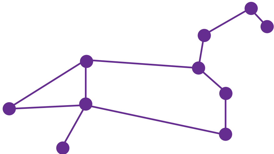
LEO (The Lion)
