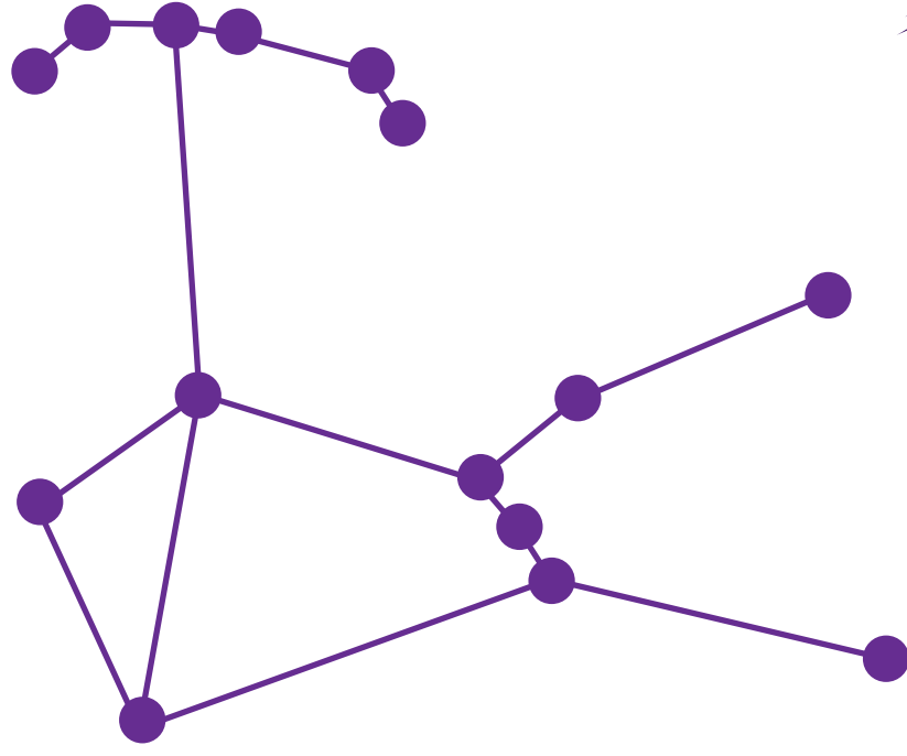
ORION (The Hunter)
