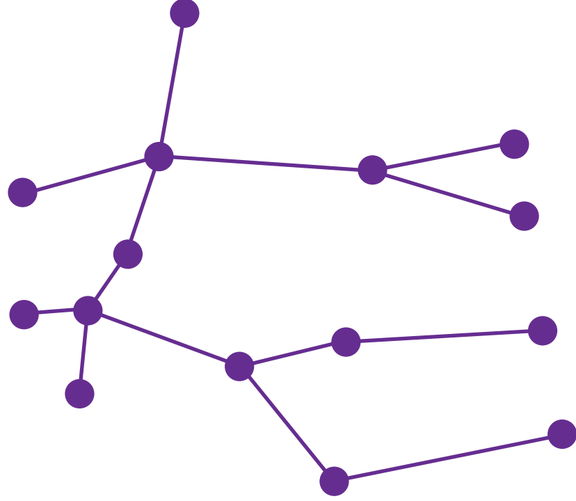
GEMINI (The Twins)
