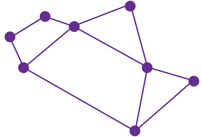
The "Teapot" Part of SAGITTARIUS (The Archer)
