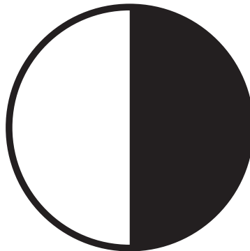
Third Quarter
