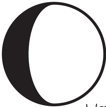
Waxing Gibbous
