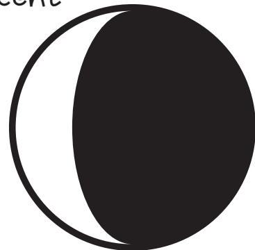
Waning Crescent
