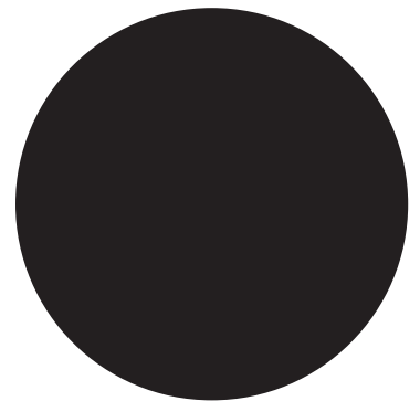
New Moon
