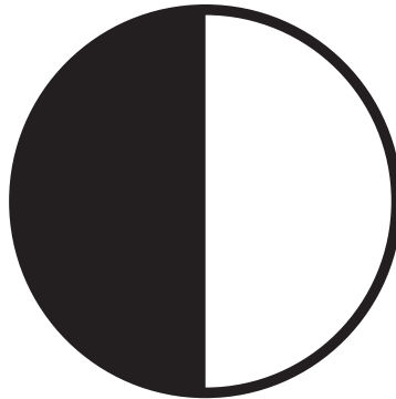
First Quarter
