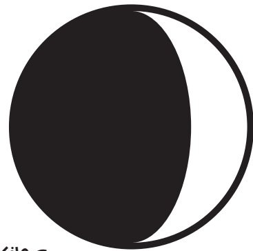
Waxing Crescent
